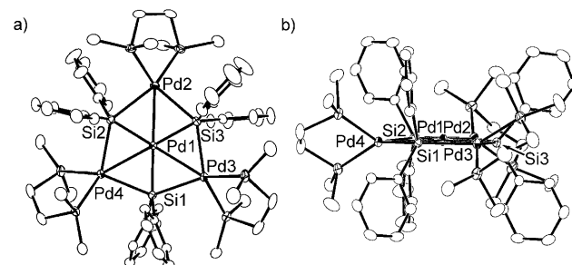
Figure 1. ORTEP representation of 2 viewed from (a) above and (b) in the plane of the \{\text{Pd}_4\text{Si}_3\} core. Thermal ellipsoids are set at 50 % probability. Hydrogen atoms and solvent molecules are omitted for clarity. Selected bond lengths [Å] and angles [°]: Pd1–Pd2 2.7122(3), Pd1–Pd3 2.7358(2), Pd1–Pd4 2.7326(2), Pd1–Si1 2.2521(8), Pd1–Si2 2.2649(8), Pd1–Si3 2.2674(8), Pd2–Si2 2.5351(8), Pd2–Si3 2.5052(8), Pd3–Si1 2.5210(6), Pd3–Si3 2.5398(8), Pd4–Si1 2.5456(7), Pd4–Si2 2.5116(8), Si1–Pd1–Si2 119.96(2), Si1–Pd1–Si3 119.88(2), Si2–Pd1–Si3 120.03(3).
